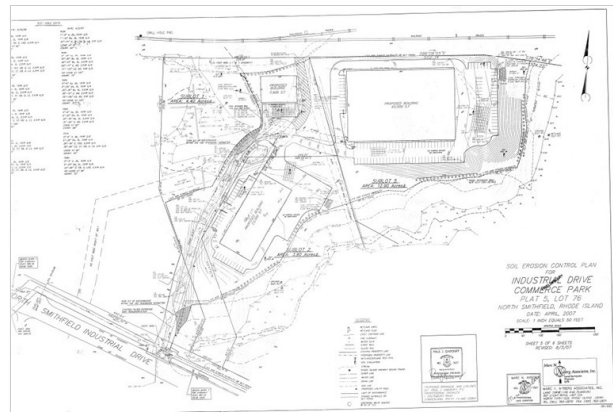
Commerce Park
